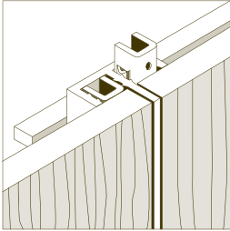
jeu = 3 mm 3 mm expansion joint Type CRP16
