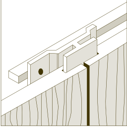
Pose à joints vifs Open butt joint installation Type H
