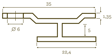
Pose à joints vifs Open butt joint installation Type H
