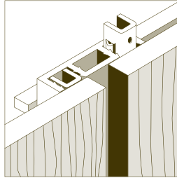
jeu max = 20 mm 20 mm max. expansion joint Type CROR
