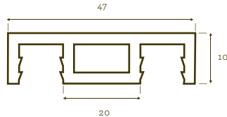
jeu max = 20 mm 20 mm max. expansion joint Type CROR
