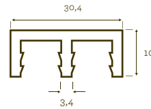
jeu max = 3,4 mm 3.4 mm max. expansion joint Type CROD
