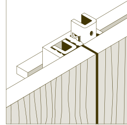
jeu max = 3,4 mm 3.4 mm max. expansion joint Type CROD
