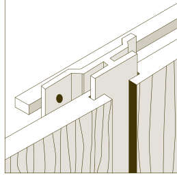
Pose à joints creux (max.6 mm) Open joint installation (6 mm max.) Type H
