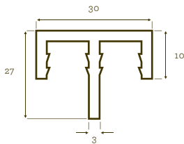
jeu = 3 mm 3 mm expansion joint Type CRP16
